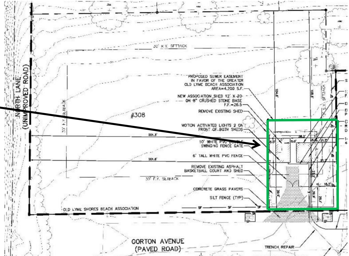
Easement Area Plan
